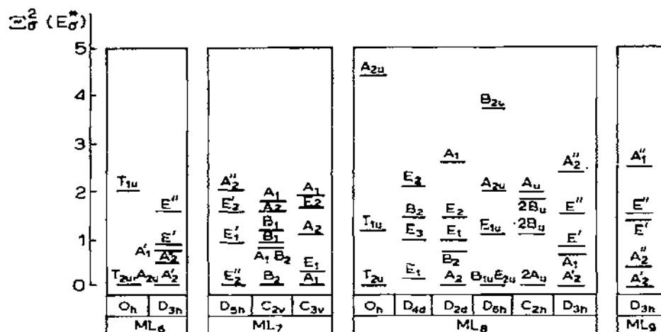
Fig. 1. Angular parameters, \Xi_{\sigma}^2 of f -orbital overlap integrals in complexes of various composition and symmetry (in E_{\sigma}^* = 7 l_0^* units) [34].
