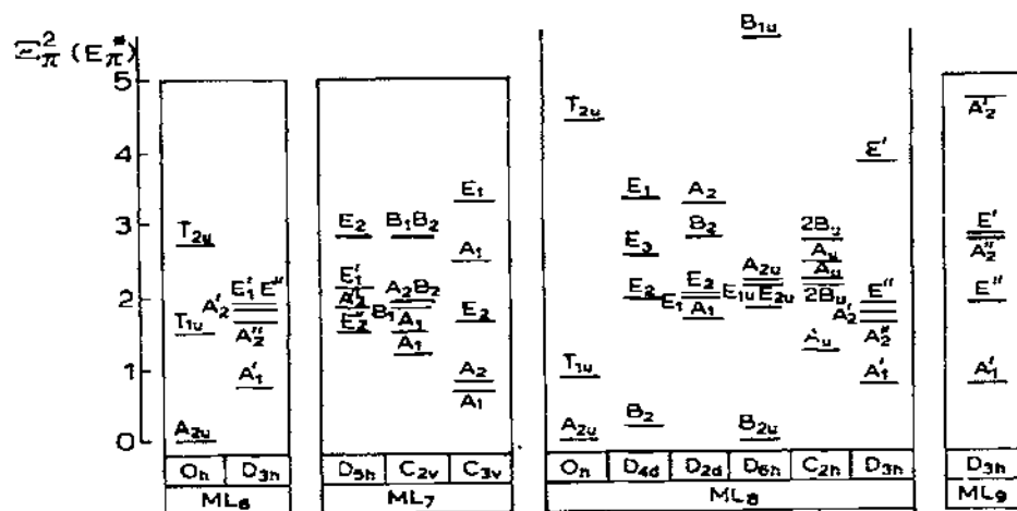
Fig. 2. Angular parameters, \Xi_{\pi}^2 of f -orbital overlap integrals in complexes of various composition and symmetry (in E_{\pi}^* = 168 e_{\pi}^* units) [34].
