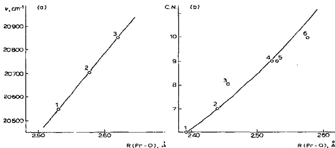
Fig. 8. (a) Dependence of {}^3P_0 \leftarrow {}^3H_4 transition energy ( \nu ) in the absorption spectra for Pr(III) complexes on mean Pr-O distances in \text{PrO}_x chromophores: (1) \text{Pr}(\text{C}_2\text{H}_5\text{SO}_4)_3 \cdot 9 \text{H}_2\text{O} [142]; (2) \text{Pr}(\text{NO}_3)_3 \cdot 6 \text{H}_2\text{O} [143]; (3) \text{Pr}_2\text{Mg}_3(\text{NO}_3)_{12} \cdot 24 \text{H}_2\text{O} [144]; ( R_{\text{Pr-O}} is determined by extrapolation from \text{Ce}_2\text{Mg}_3(\text{NO}_3)_{12} \cdot 24 \text{H}_2\text{O} [145]). (b) Interrelation between praseodymium coordination numbers (CN) and \bar{R}(\text{Pr-O}) : (1) \text{C-Pr}_2\text{O}_3 [146]; (2) \text{Pr}_2(\text{dpm})_6 [137]; (3) \text{NH}_4\text{Pr}(\text{tta})_4 [138]; (4) \text{Pr}_2(\text{C}_2\text{O}_4)_3 \cdot 10 \text{H}_2\text{O} [139]; (5) \text{Pr}(\text{C}_2\text{H}_5\text{SO}_4)_3 \cdot 9 \text{H}_2\text{O} [140]; (6) \text{Pr}(\text{NO}_3)_3 \cdot 6 \text{H}_2\text{O} [141].
