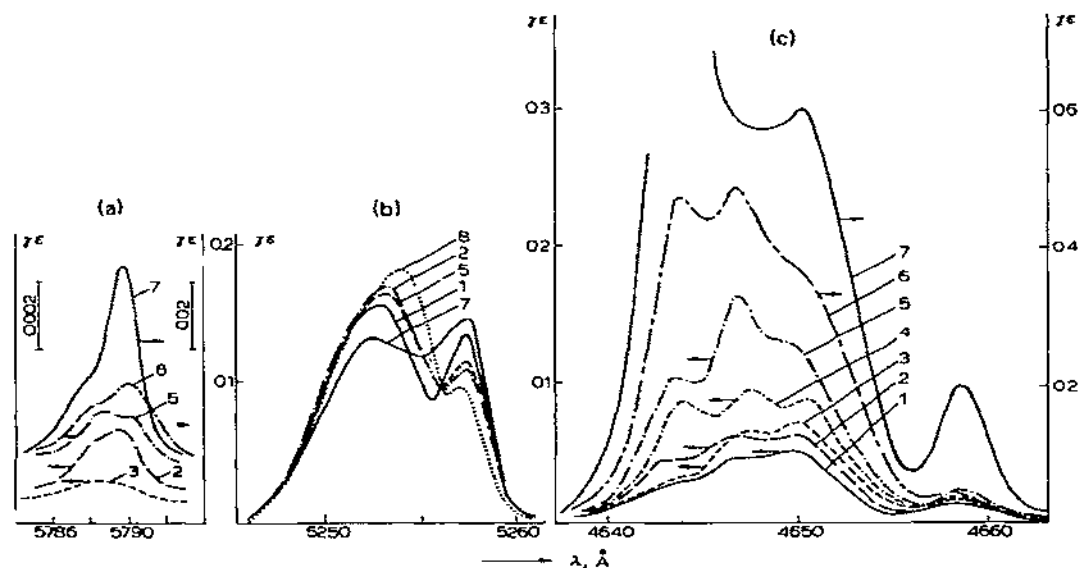
Fig. 11. Absorption spectra of Eu(III) salt solutions in transitions: (a) {}^5D_0 \leftarrow {}^7F_0 ; (b) {}^5D_1 \leftarrow {}^7F_0 ; (c) {}^5D_2 \leftarrow {}^7F_0 [191]. (1) 0.036 M \text{Eu}(\text{ClO}_4)_3 ; (2) 1 M \text{EuCl}_3 ; (3) 1 M \text{Eu}(\text{ClO}_4)_3 ; (4) 0.10 M \text{Eu}(\text{ClO}_4)_3 in 5 M \text{LiCl} ; (5) 1 M \text{Eu}(\text{BrO}_3)_3 ; (6) 0.10 M \text{Eu}(\text{ClO}_4)_3 in 0.4 M \text{KCNS} ; (7) 0.10 M \text{Eu}(\text{ClO}_4)_3 in 10 M \text{LiCl} ; (8) 0.10 M \text{Eu}(\text{ClO}_4)_3 in 8 M \text{NaClO}_4 .
